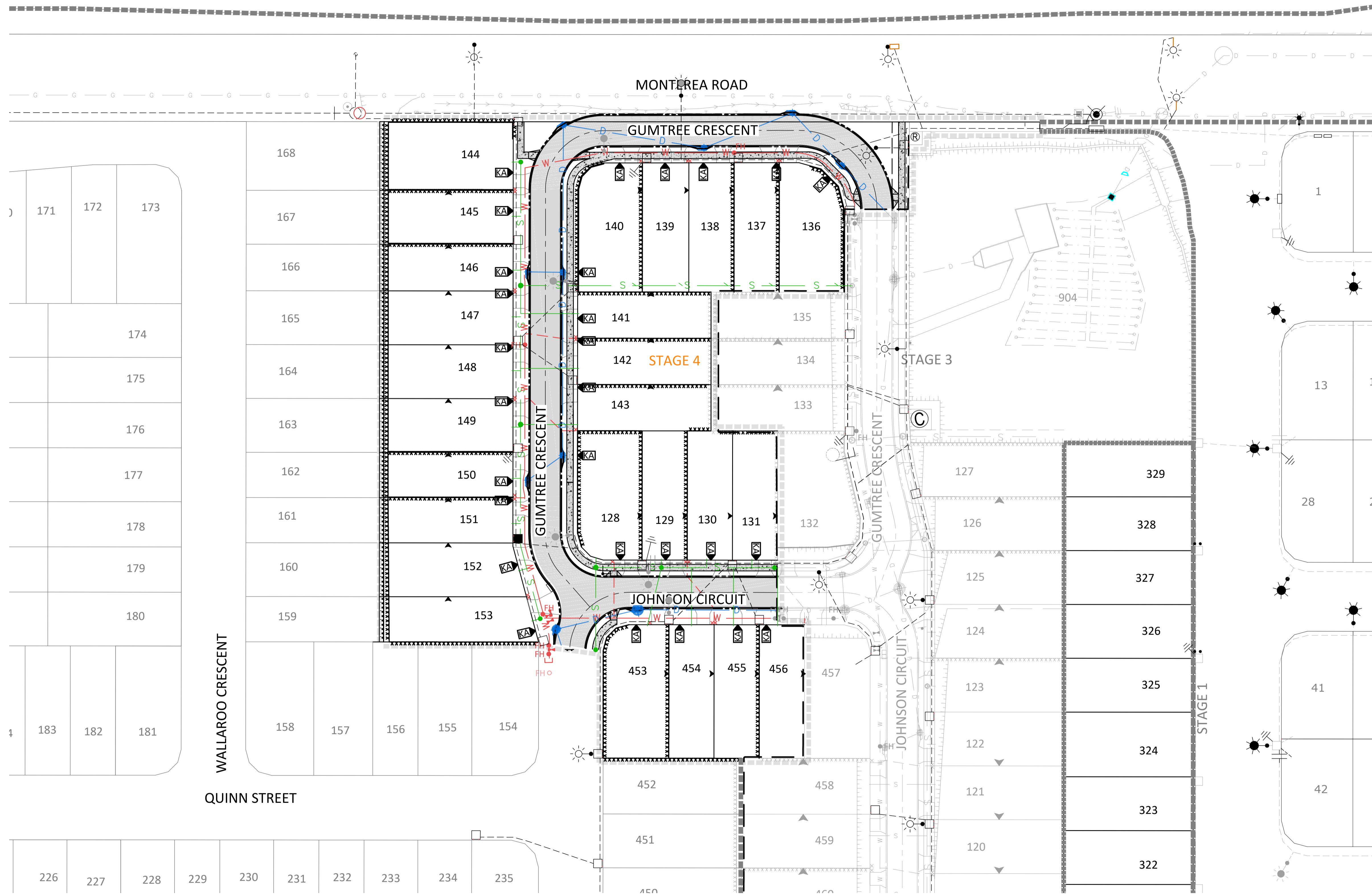
PLAN SCALE 1:500
