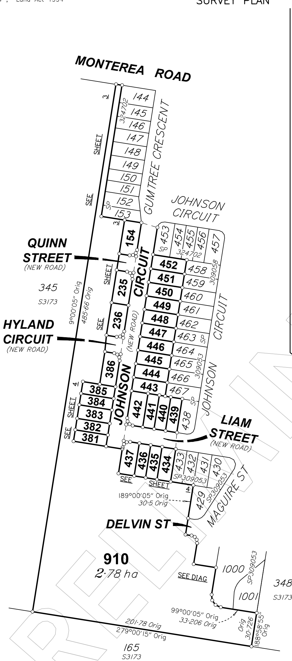
DIAGRAM SCALE 1: 600
