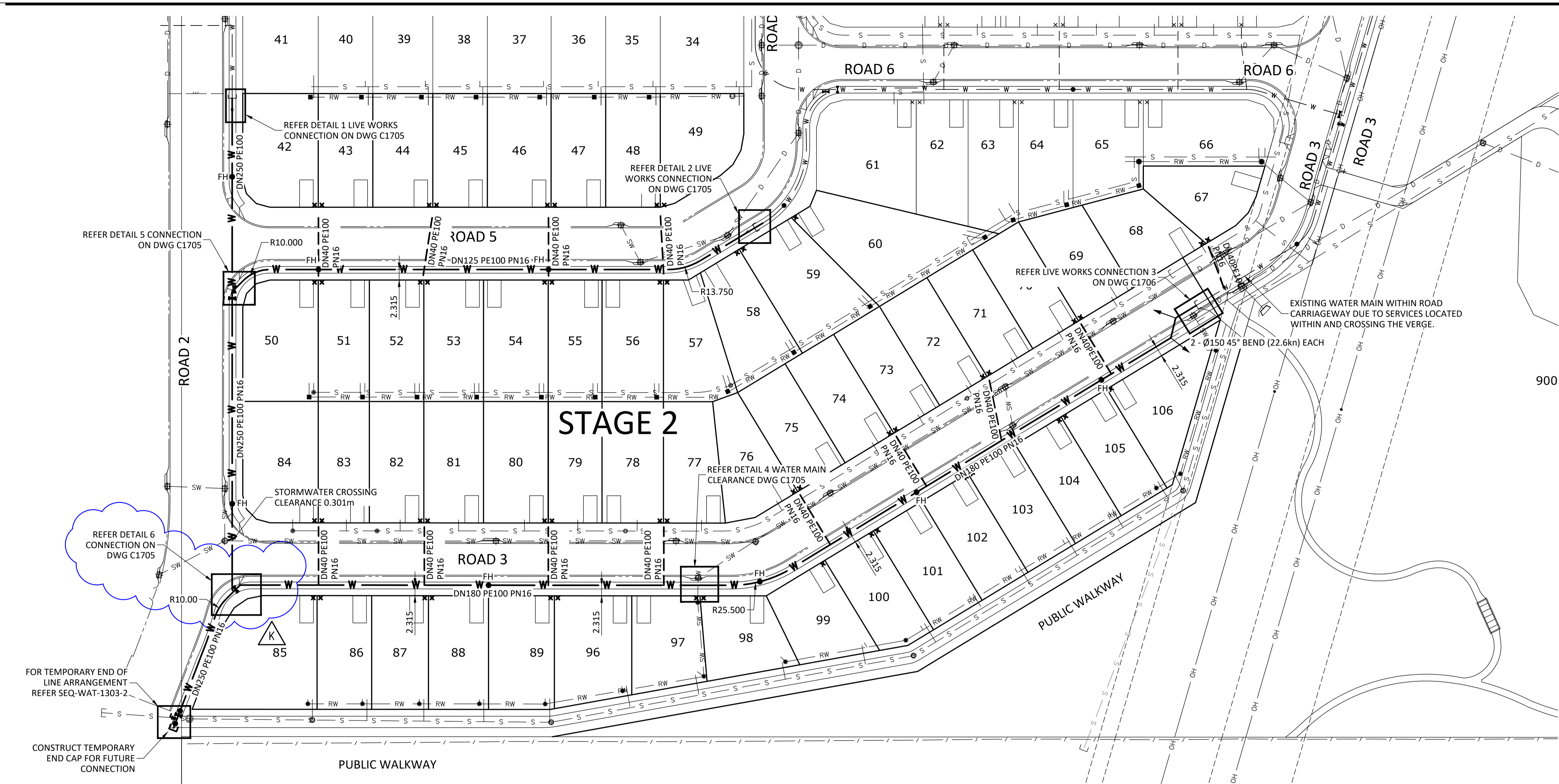
PLAN SCALE:1:500
